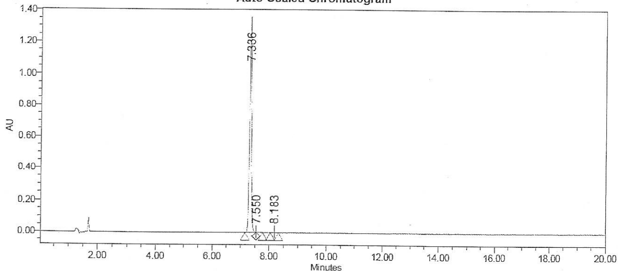
Auto-Scaled Chromatogram
